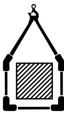
BASKET HITCH
